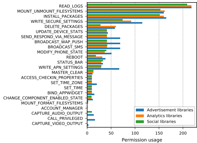
Figure 4: System permissions requested by pre-installed apps embedding TPLs.
