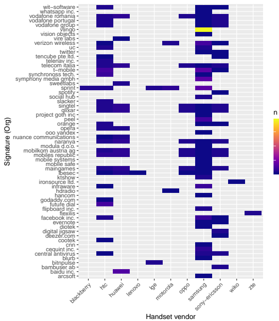
Figure 3: Apps accessing vendors’ custom permissions.
